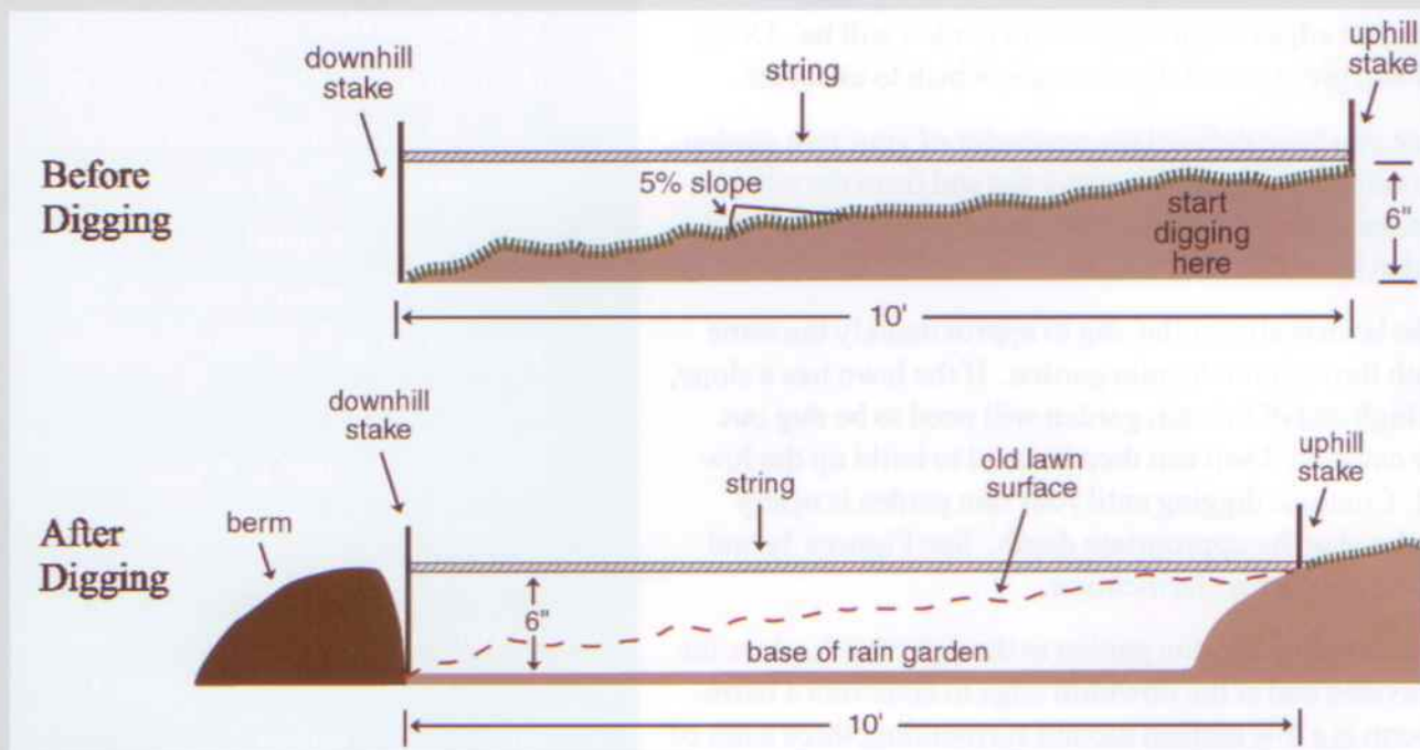
Figure 3a - Between 3% and 8% slope lawn
