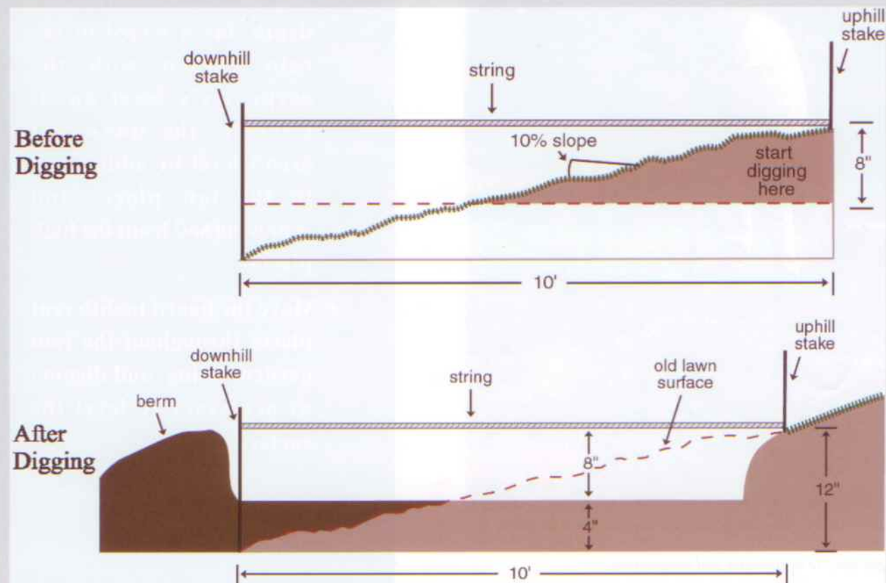
Figure 3b - Between 8% and 12% slope lawn
