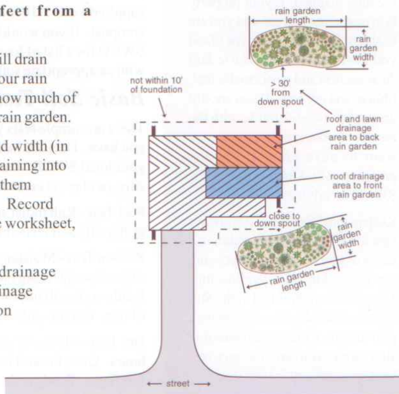
Figure 1 - Rain gardens can be placed near your home or further out in your yard.
